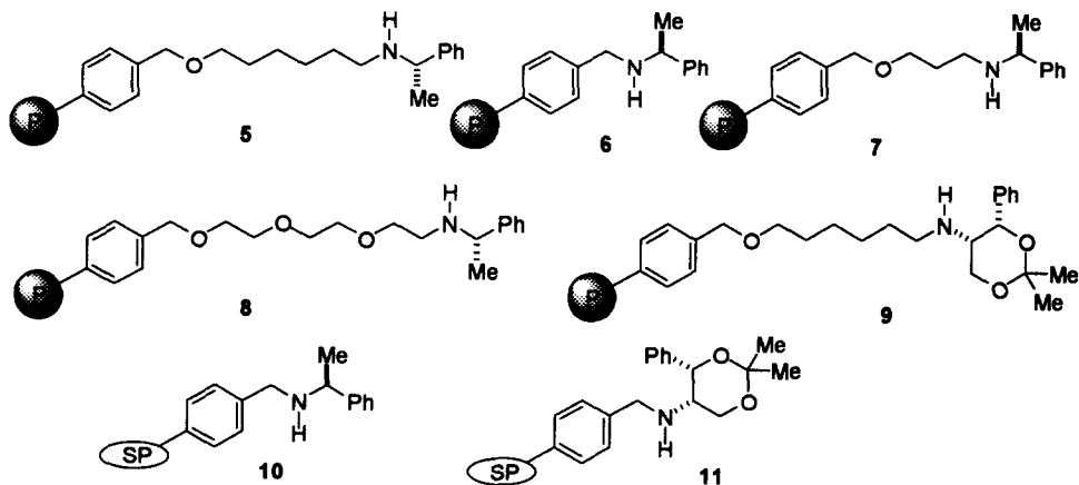
Figure 1. Structures of chiral amines on insoluble (P) and soluble (SP) polymer support
